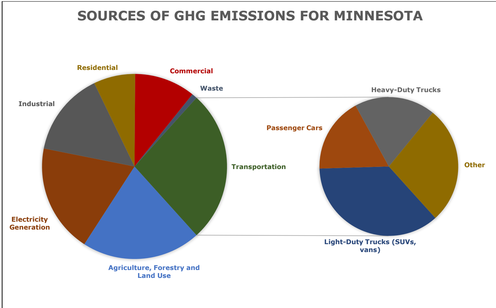
Figure 3.4: Sources of Emissions (2020). *Other includes air conditioning, aviation, buses, marine, motorcycle, natural gas transmission, off-highway, railroad, and recreational vehicles.
