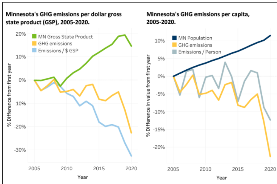
Figure 3.12: (Left) - Minnesota's Emissions per Dollar Gross State Product (GSP), 2005-2020. (Right) - Minnesota's GHG Emissions Per Capita, 2005-2020 Data courtesy from MPCA's Greenhouse Gas Emissions Inventory 2005-2020 Report.
