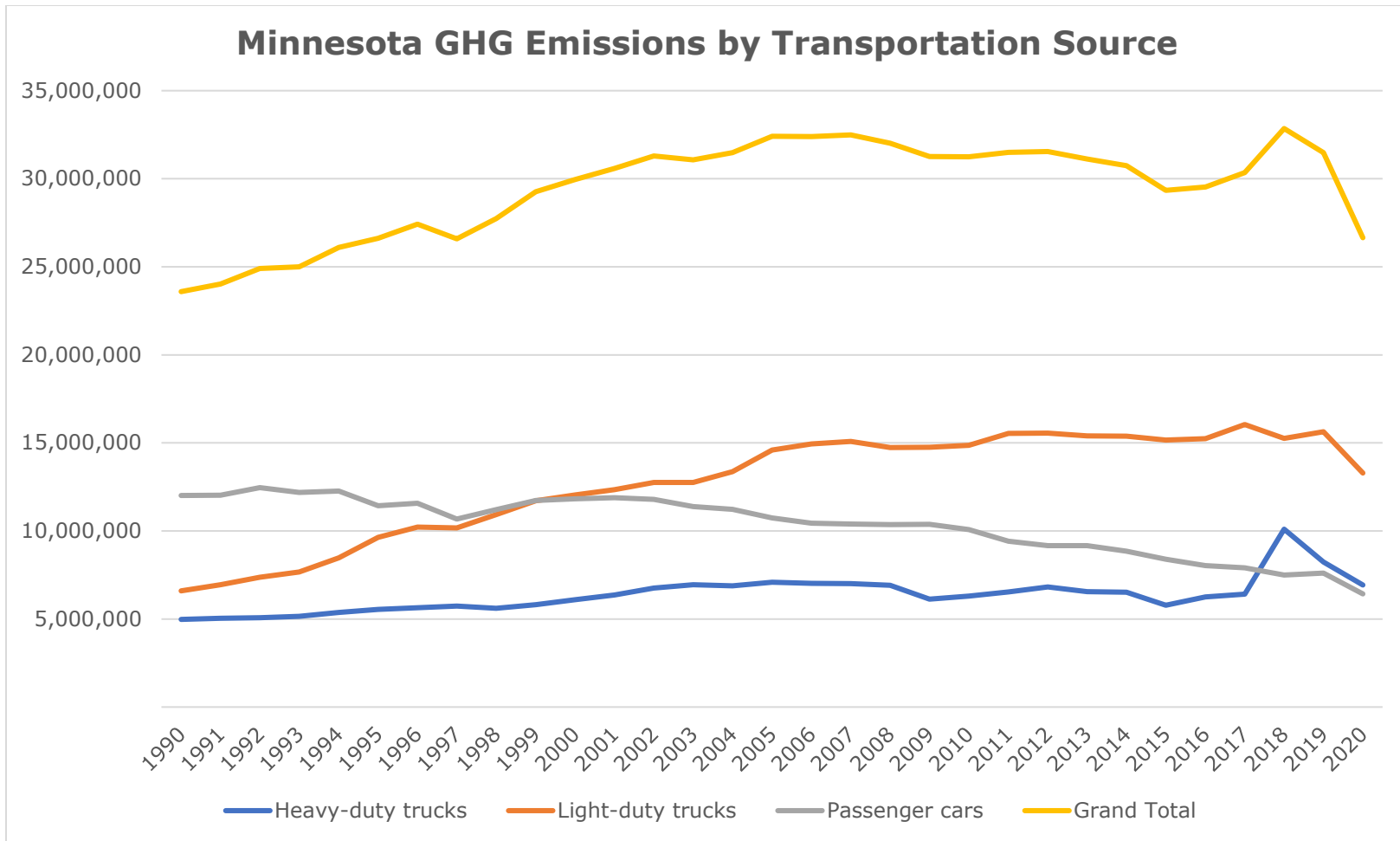
Figure 3.5: Emissions by Transportation Source in Minnesota.
