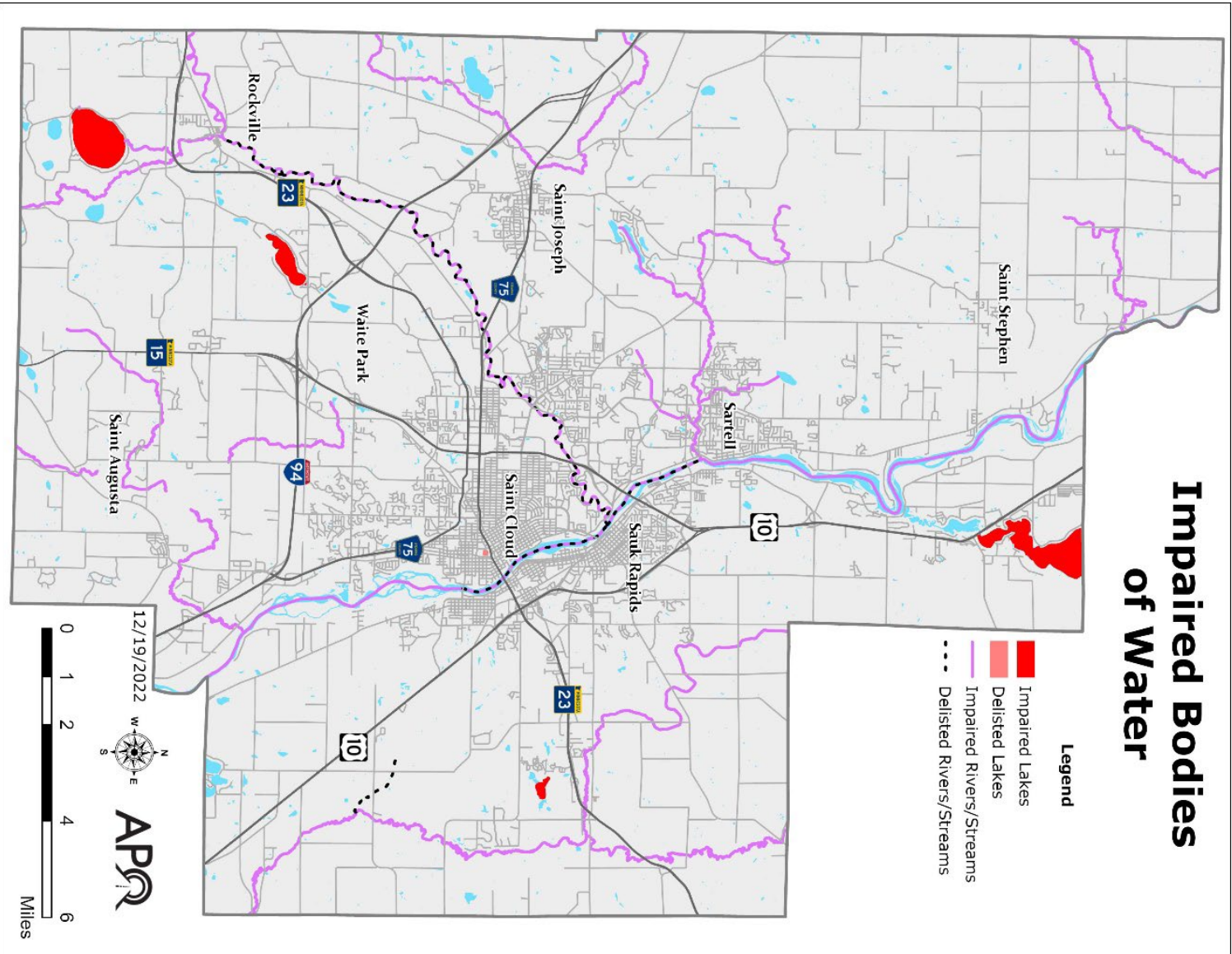
Figure 3.39: Impaired Bodies of Water. Data courtesy of MPCA.
